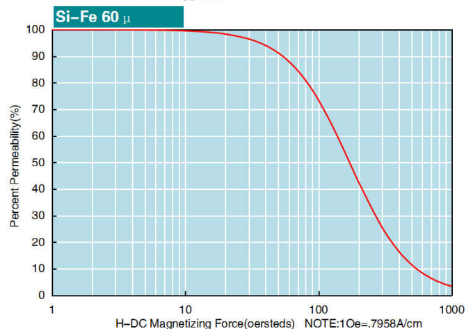
DC-Bias Curves(Typical)
